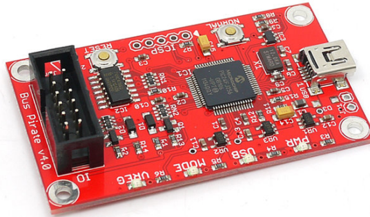
Figure 3.2: Bus Pirate v.4 (photo taken from [1])
